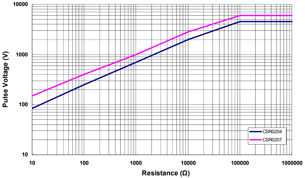
1.2/50μs Lightning Surge
